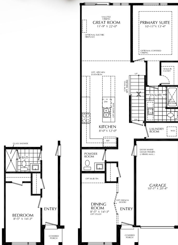
Opt. Bedroom Layout
