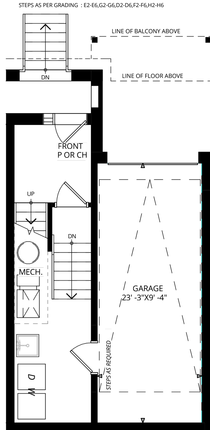
FIRST FLOOR
