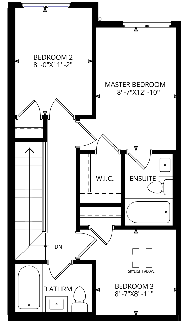
THIRD FLOOR
