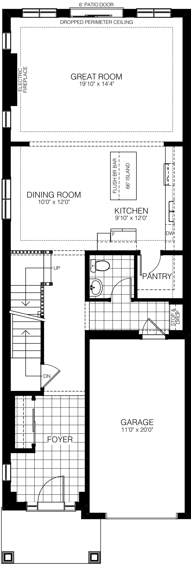
MAIN FLOOR ELEV. B
