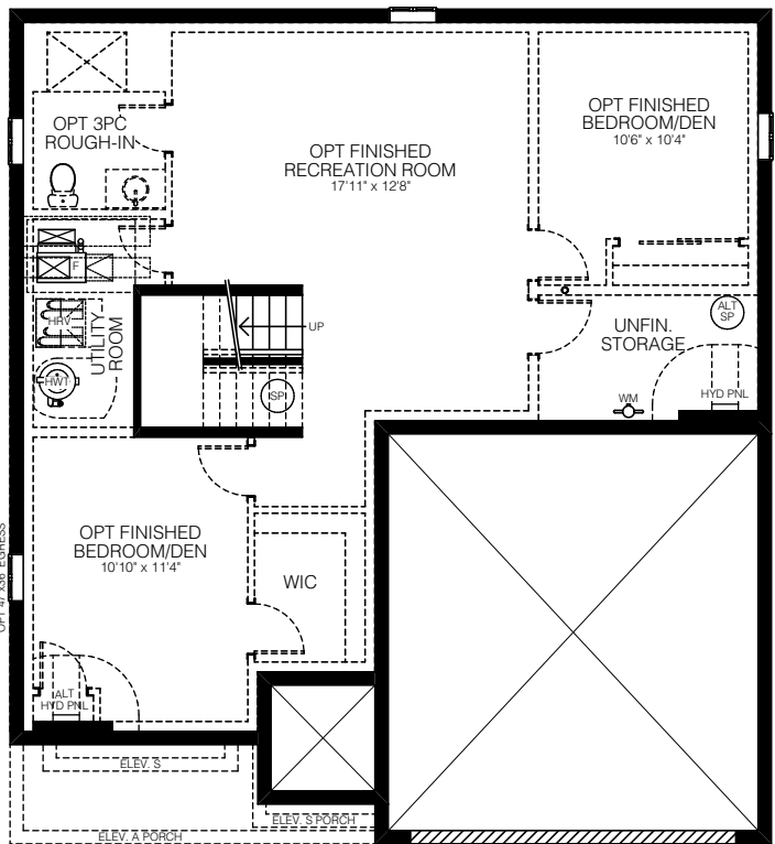
BASEMENT
