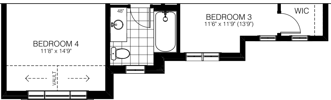
SECOND FLOOR ELEV. B
