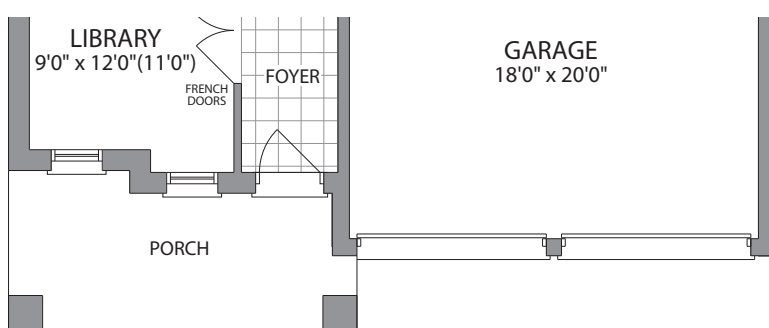
GROUND FLOOR ELEVATION B
