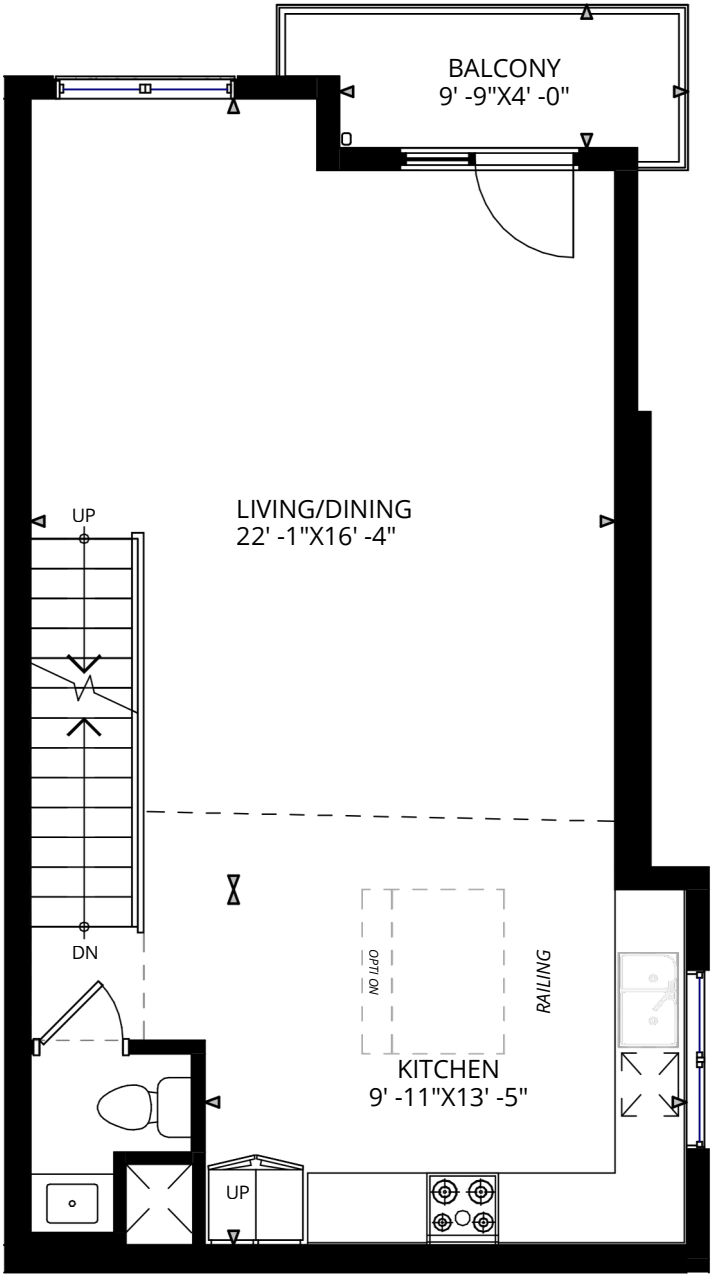
SECOND FLOOR
