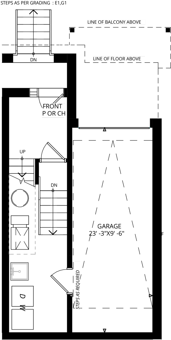
FIRST FLOOR
