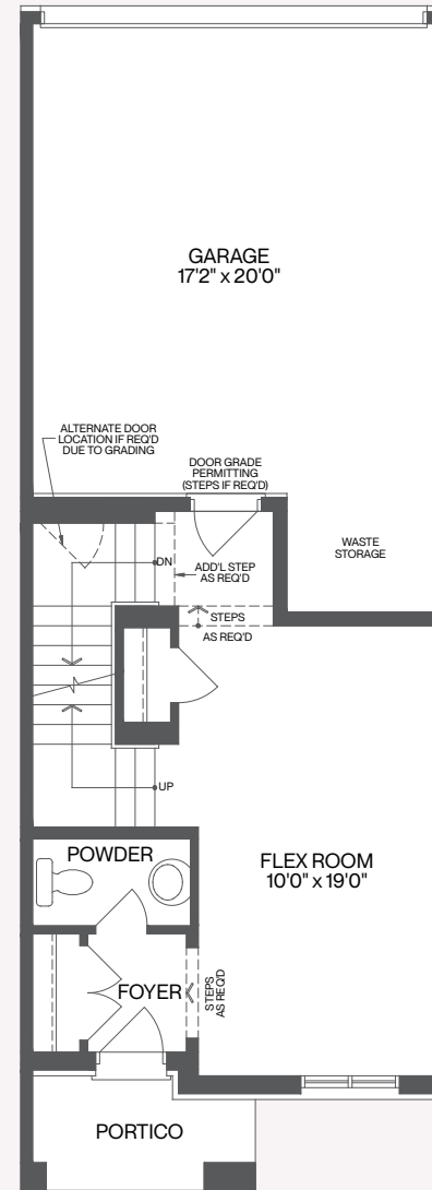
Ground Floor Plan, El. 'A & B'
