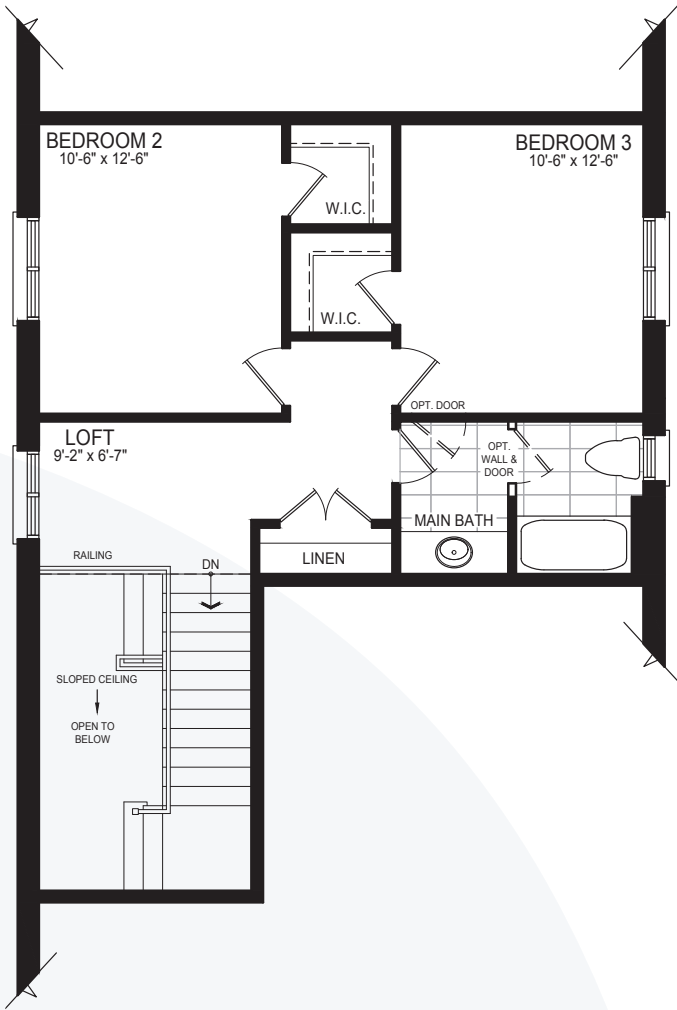
LOFT FLOOR Style B
