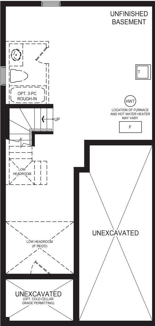
BASEMENT Style C
