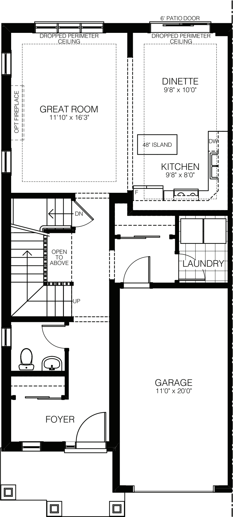
MAIN FLOOR ELEV. A1/A2
