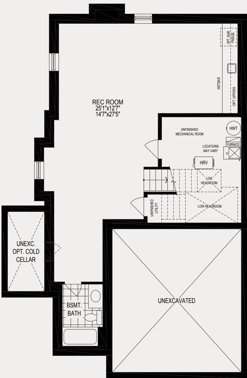
ENTERTAINER'S RETREAT OPTION +816 SQ. FT.
