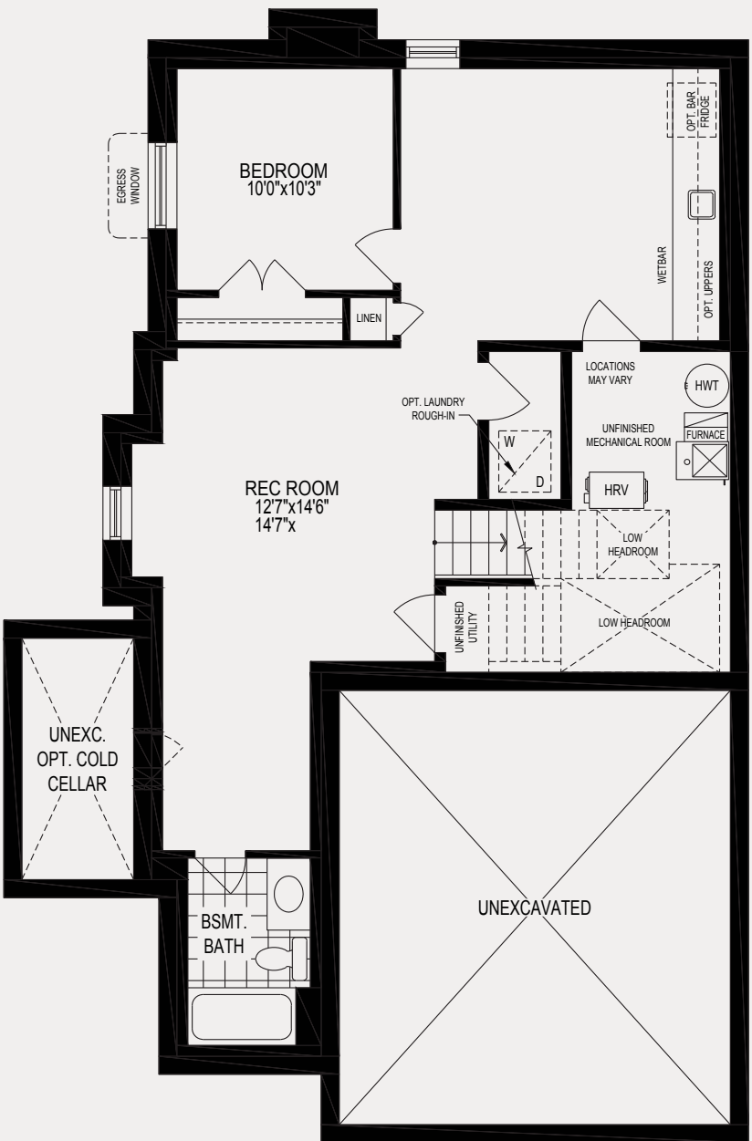
FAMILY FLEX SUITE OPTION +844 SQ. FT.
