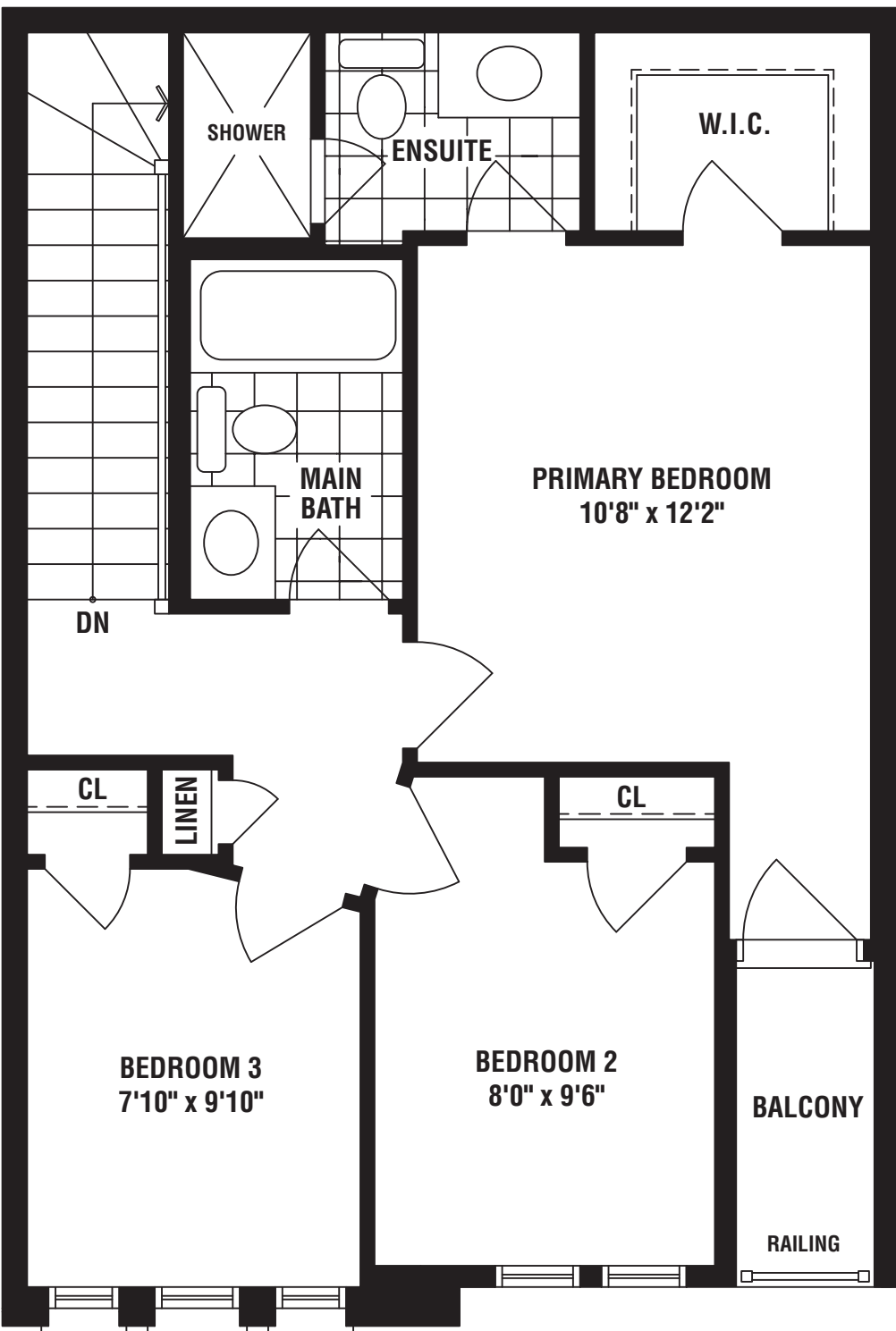
UPPER LEVEL PLAN ELEV. 'A'
