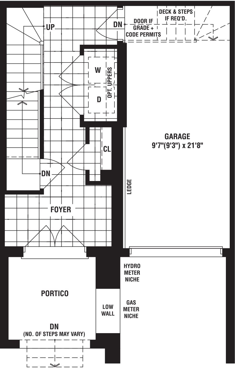
LOWER LEVEL PLAN ELEV. 'A'
