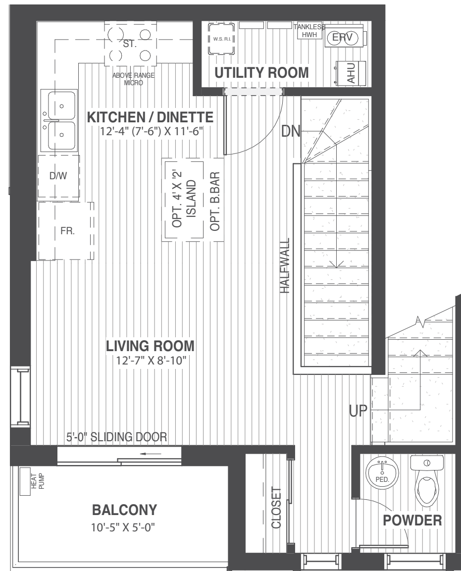
SECOND FLOOR LEVEL
