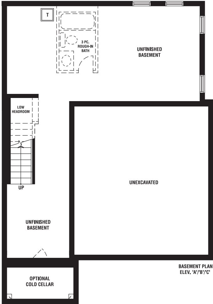
PARTIAL BASEMENT PLAN OPT. WALK UP BASEMENT CONDITION (SUBJECT TO GRADING APPROVAL) (LOCATION MAY VARY)
