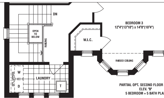
OPT. SECOND FLOOR PLAN ELEV. 'A' (5 BEDROOM + 5 BATH)
