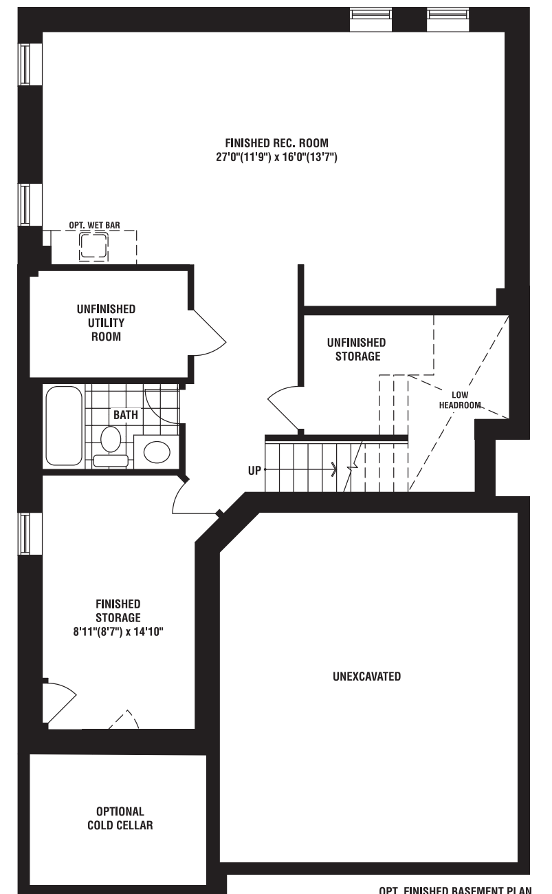
OPT. FINISHED BASEMENT PLAN ELEV. 'A'/B'/C' (OPT. FIN. BASEMENT 768 SF)
