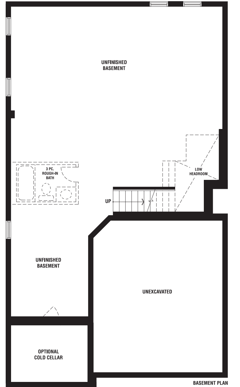
BASEMENT PLAN ELEV. 'A'/B'
