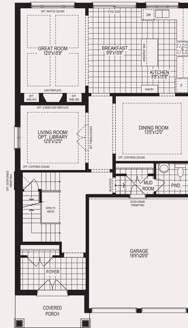
OPT. GROUND FLOOR PLAN A W/ LIVING ROOM/LIBRARY
