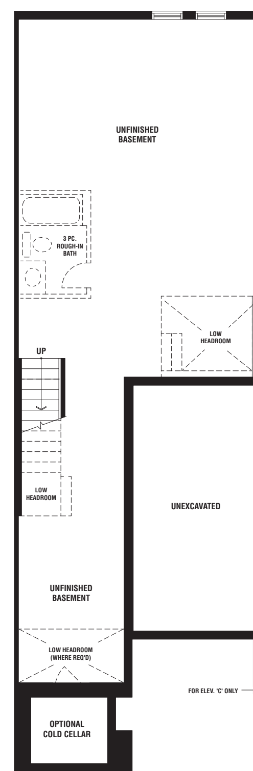
FOR ELEV. 'C' ONLY BASEMENT PLAN ELEV. 'B'/'C'
