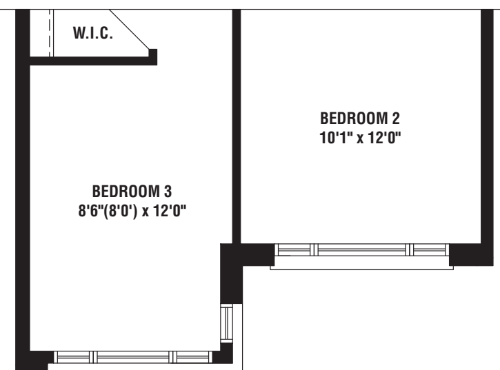
PARTIAL OPT. SECOND FLOOR PLAN ELEV. 'C' (4 BEDROOM)
