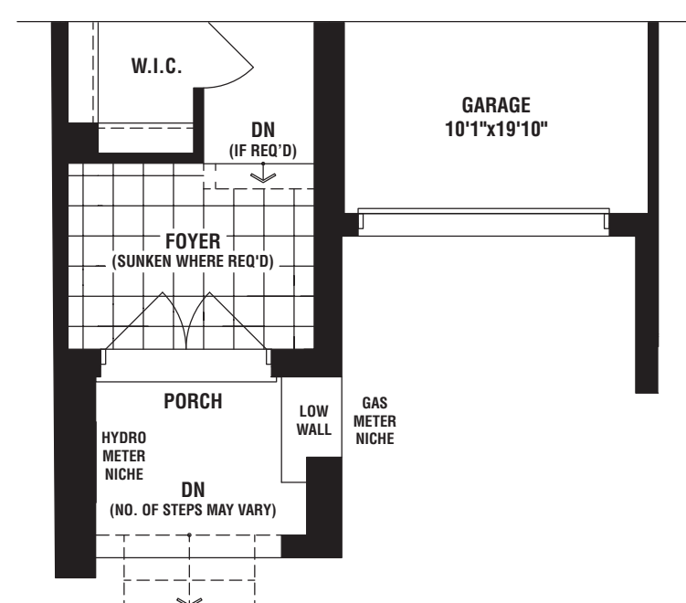
PARTIAL GROUND FLOOR PLAN ELEV. 'C'
